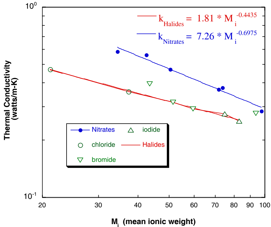
Fig. 12. Thermal conductivity correlation in one-component nitrate and halide salts [27, 28].
