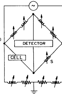
F. CAREY-FOSTER BRIDGE (48) (CELL AND S ARE INTER- CHANGEABLE)
