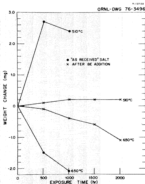
Fig. 5. Weight Change Results for Type 316 Stainless Steel Specimens Exposed to \text{LiF}-\text{BeF}_2 Salt in Both the As-Received Relatively Oxidizing Condition and in the Relatively Reducing Condition Created by the Addition of Beryllium to the Salt.
